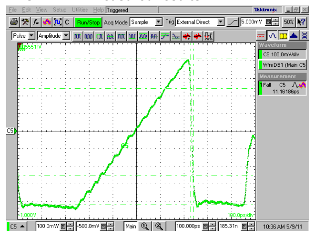
Example: 16 step ramp @ 34 GS/s
